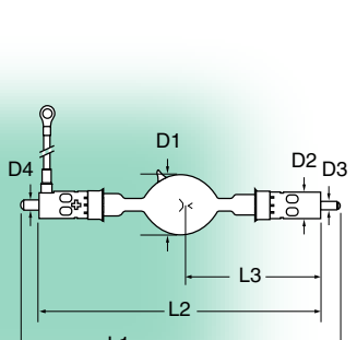
UXL-70SC
