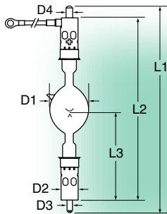
UXL-20SC
