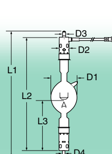
UXL-60SC UXL-50SC
