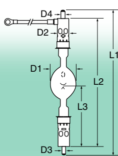
UXL-30SC
